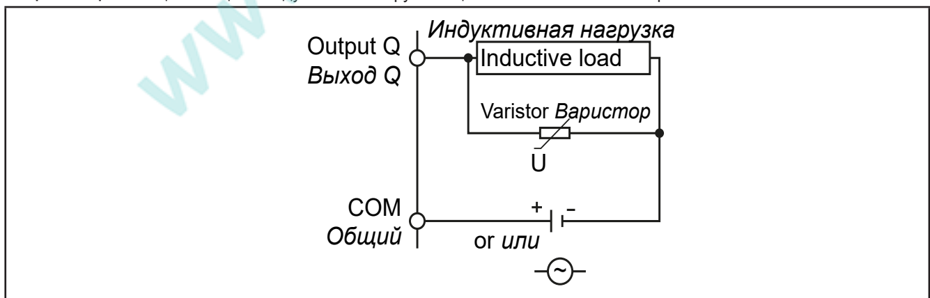
Рис. 14. Protection circuit C
