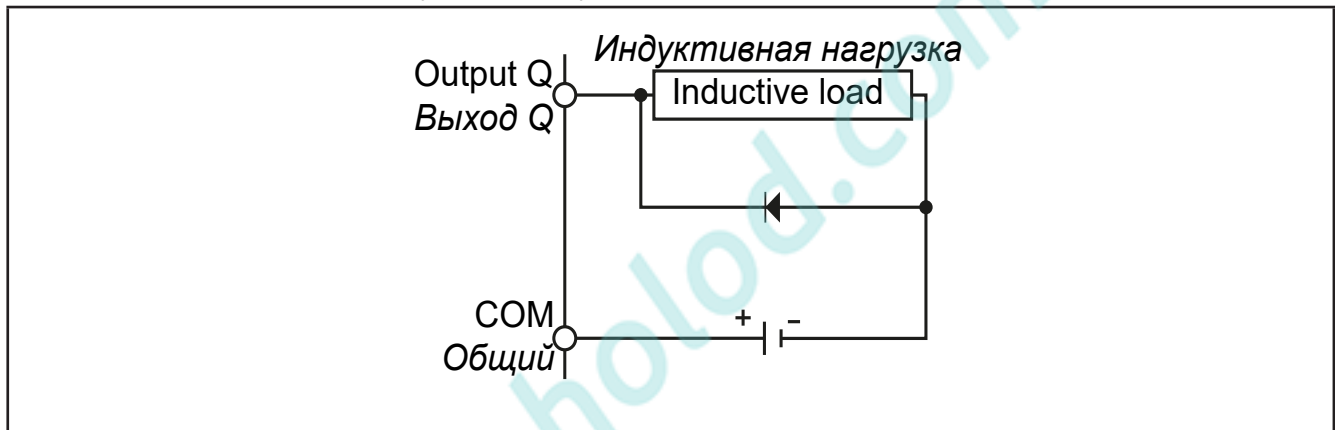
Рис. 13. Protection circuit B
